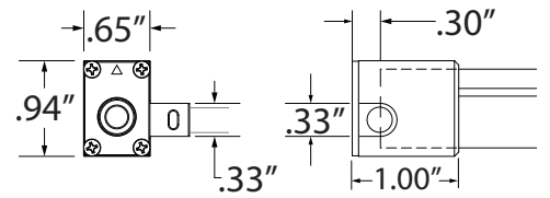
TRACE LEAD - SIDE Horizontal Side Lead Entry 5' Power Lead Cable with End Cap
